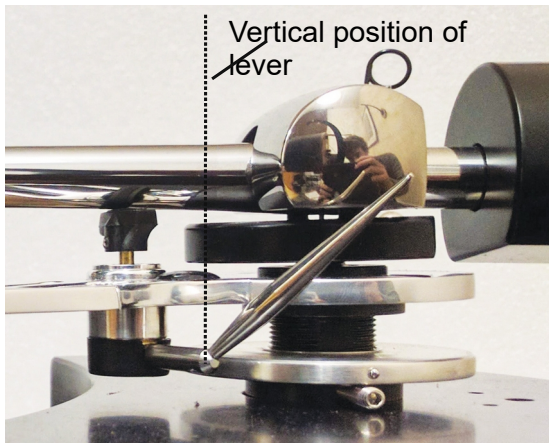
Photo showing lift / lower lever raised past vertical
